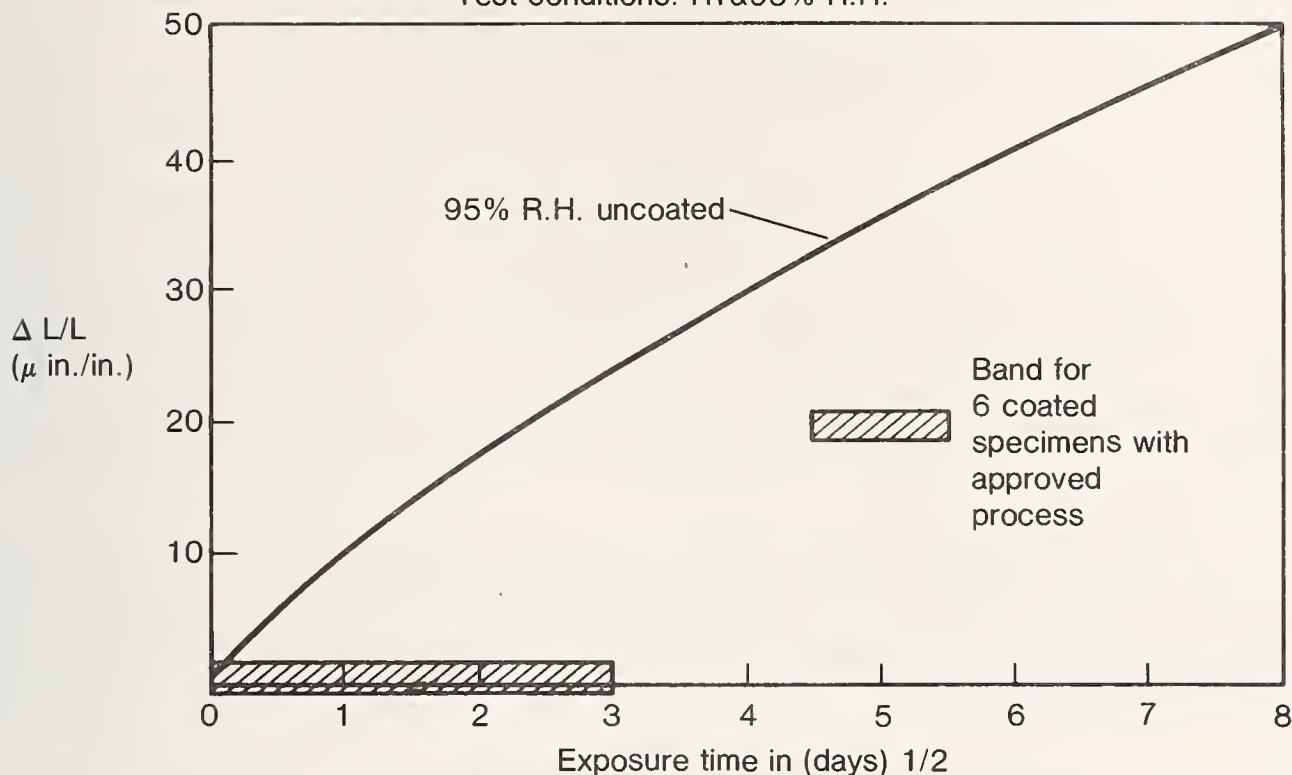
Figure 4. Dimensional stability study of six graphite/epoxy specimens (January 30 to February 8, 1977).
